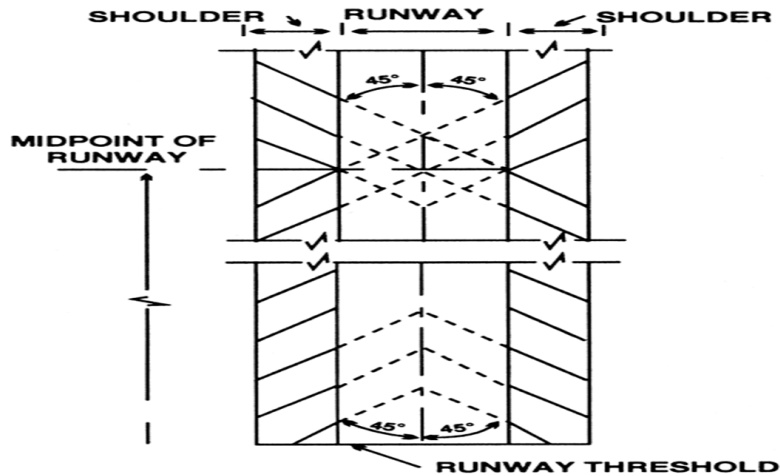
Figure 3.1. Runway Shoulder Markings.
