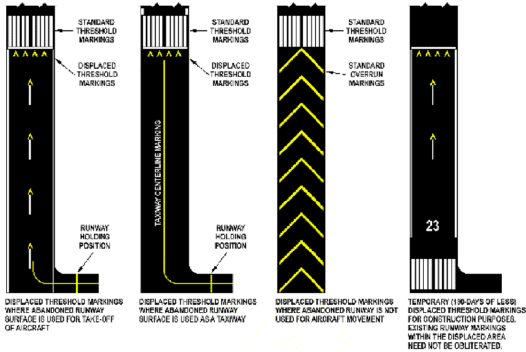
Figure 3.3. USAF Threshold Markings.
