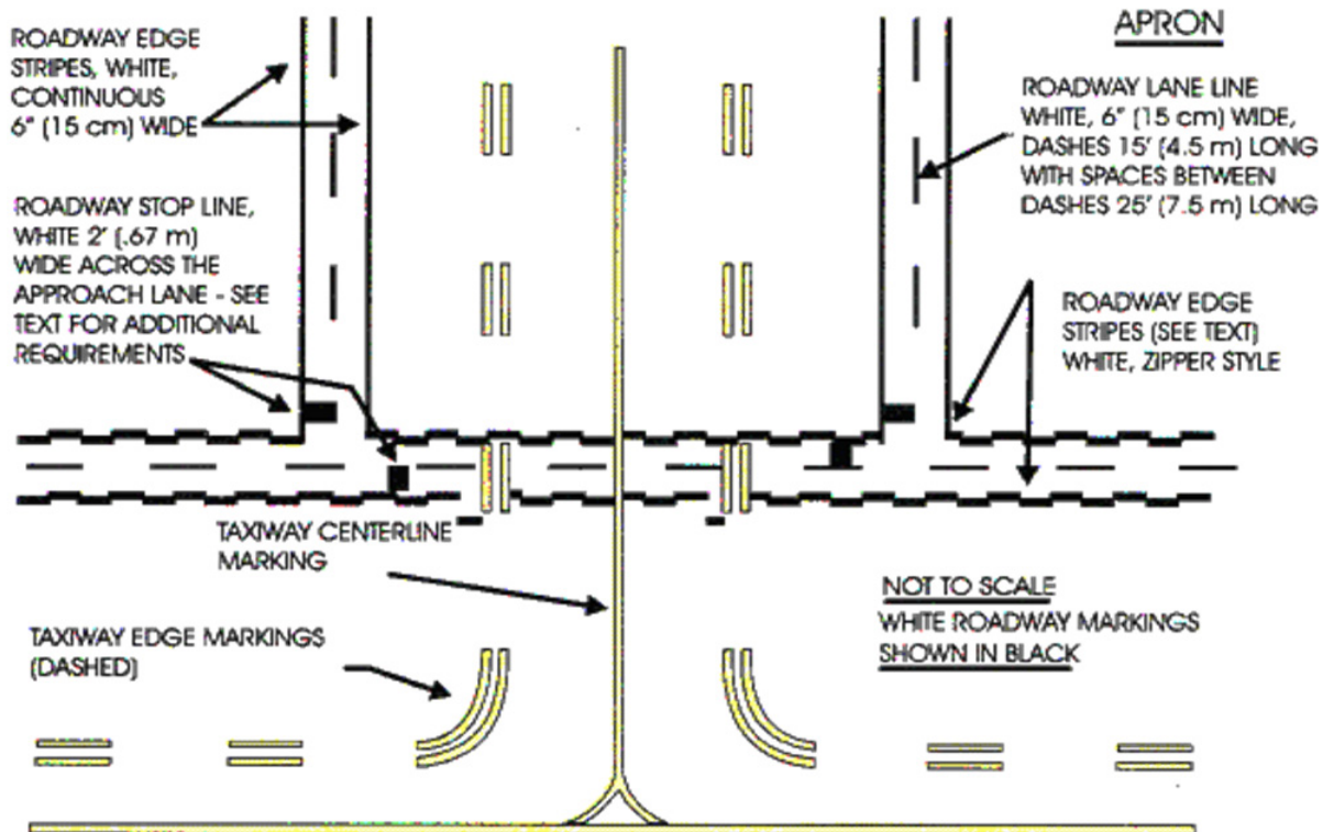
Figure 3.13. Vehicle Roadway Markings.
