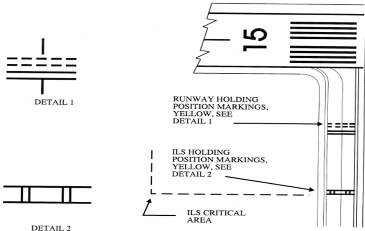
Figure 3.10. Holding Position Markings for ILS Critical Area.
