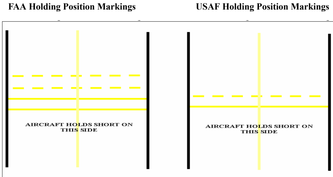
Figure 3.9. Runway Holding Position Markings.
