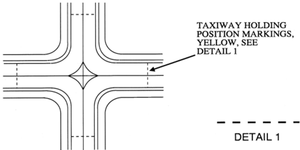
Figure 3.11. Holding Position Markings for Taxiway/Taxiway Intersections.
