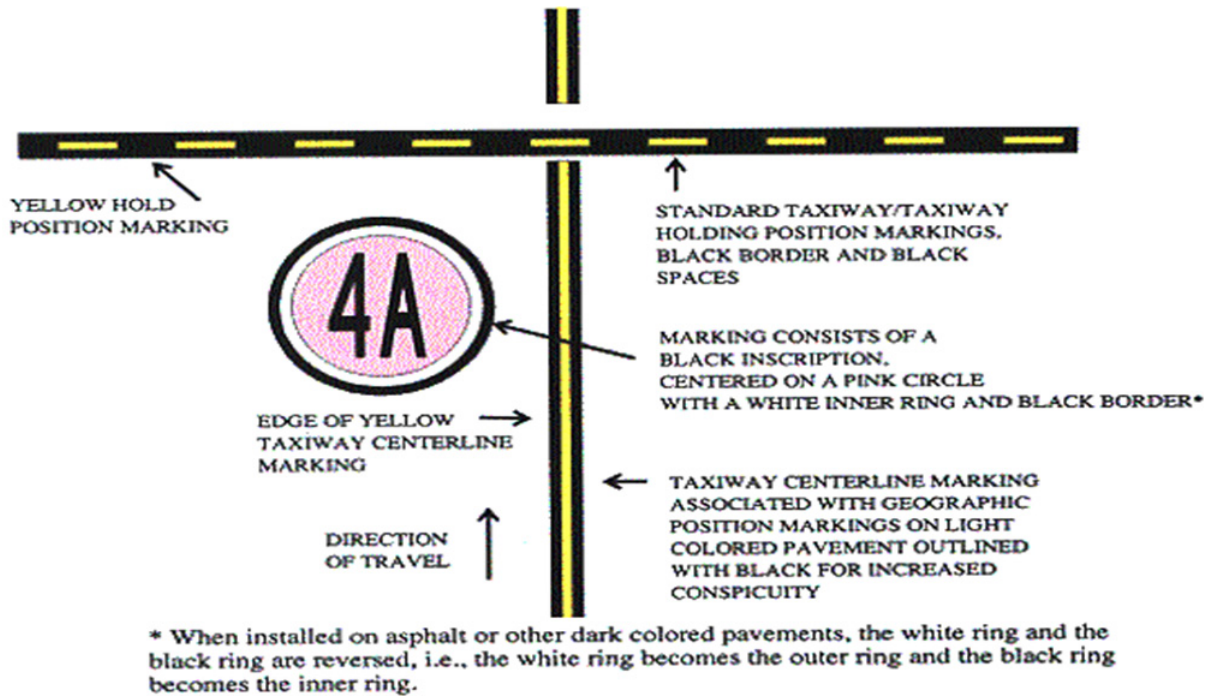
Figure 3.8. Geographic Position Markings.
