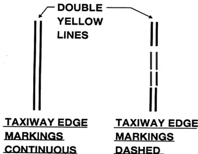
Figure 3.5. Taxiway Edge Markings.
