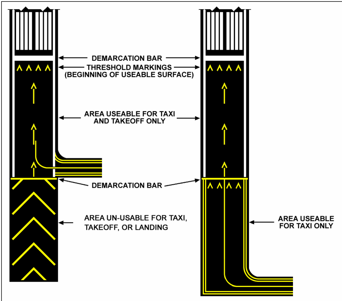
Figure 3.2. FAA Demarcation Bars and Threshold Markings.
