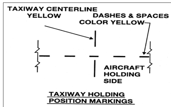
Figure 3.4. Taxiway Holding Position Markings.
