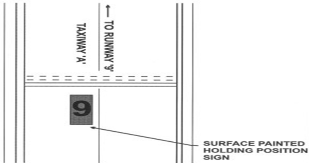
Figure 3.12. Surface Painted Holding Position Sign.
